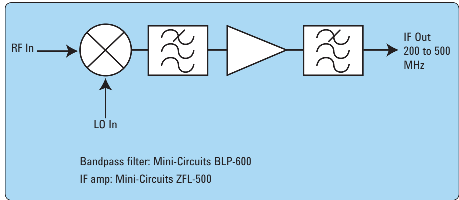
Figure 13. Block diagram of suggested downconverter. See Table 8 for further details.
